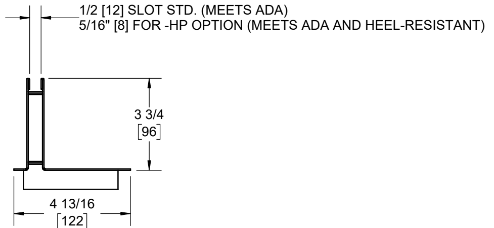
END VIEW
