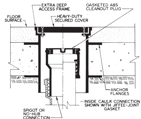
58680-CO3 Series Access Frame and Cover with 3" cast iron ferrule shown installed in an unfinished floor at grade level.
