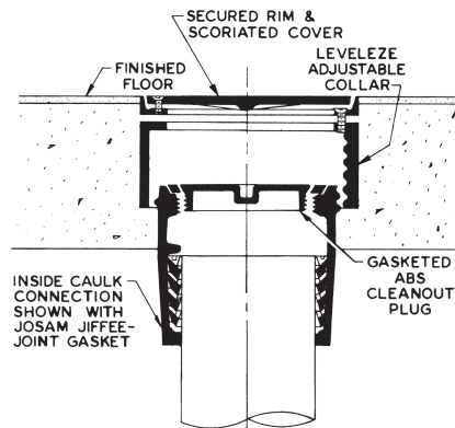
57000 Series KLEENATRON® Cleanout with LEVELEZE® adjustable collar shown installed in a finished floor.
